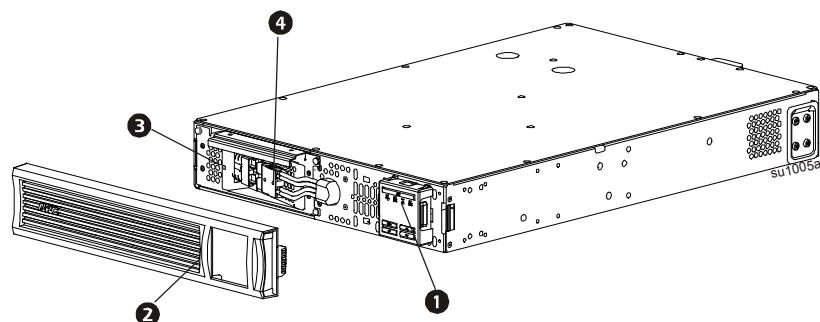
Rackmontage SMT2200RM2UC, SMT2200RM12UC, SMT3000RM2UC en SMT3000RM12UC
