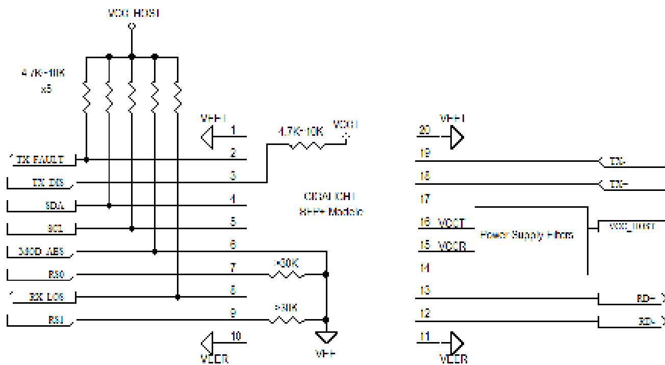
Figure4. Host-Module Interface
