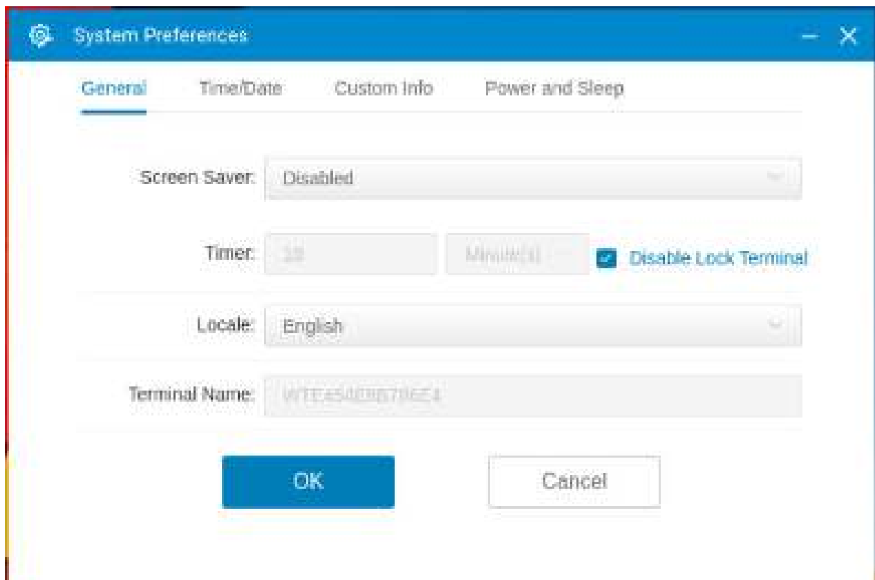
Figure 37. General tab
