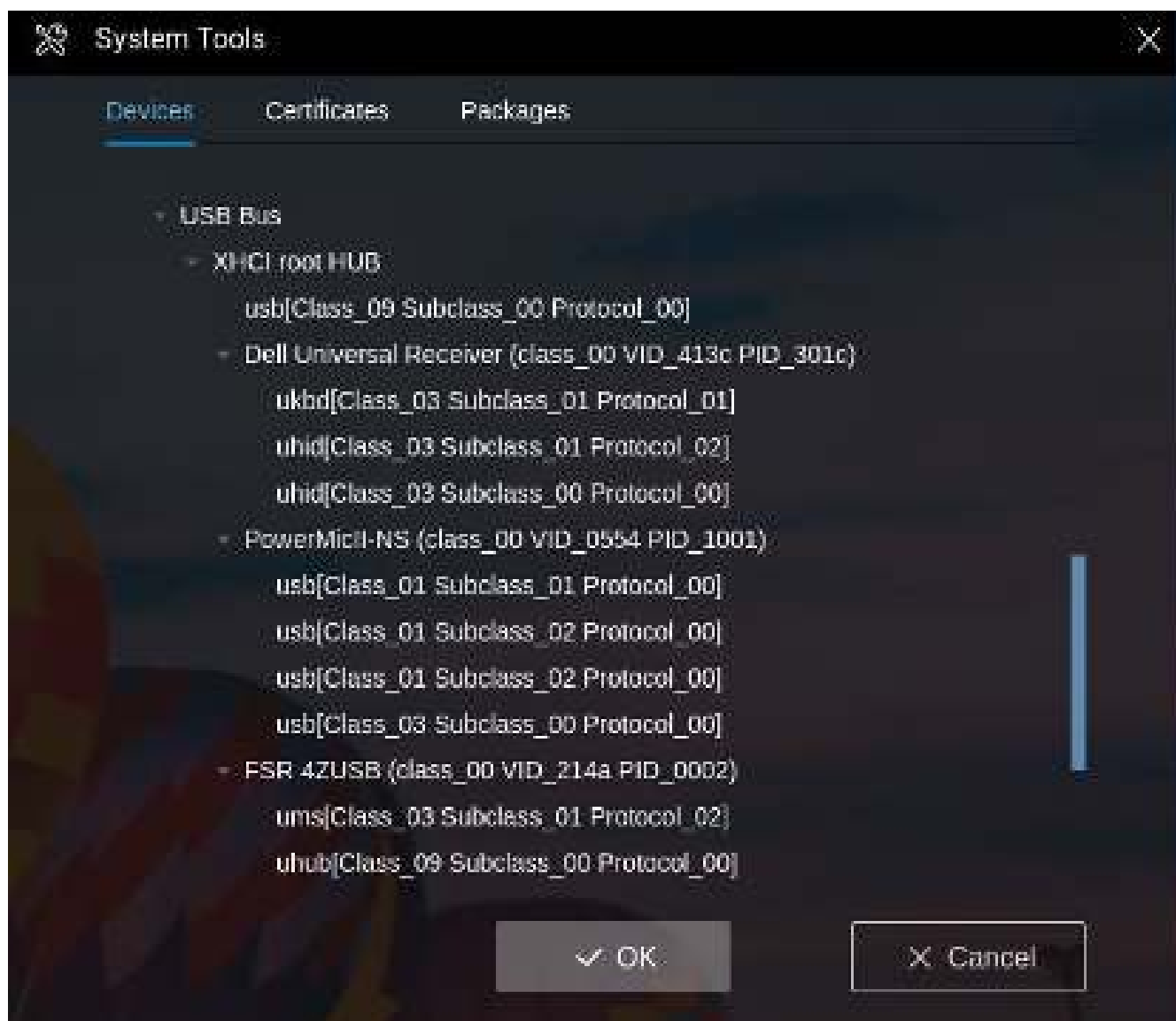
Figure 26. USB redirection
