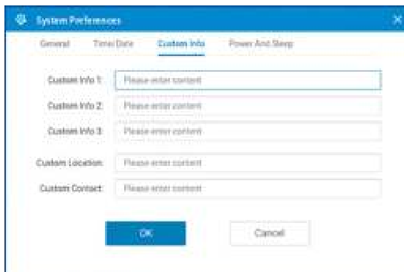
Figure 39. Custom information
