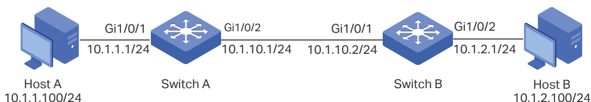
Figure 9-1 Network Topology
