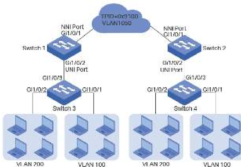
Figure 4-1 Network Topology
