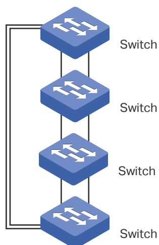
Figure 4-2 Ring Topology
