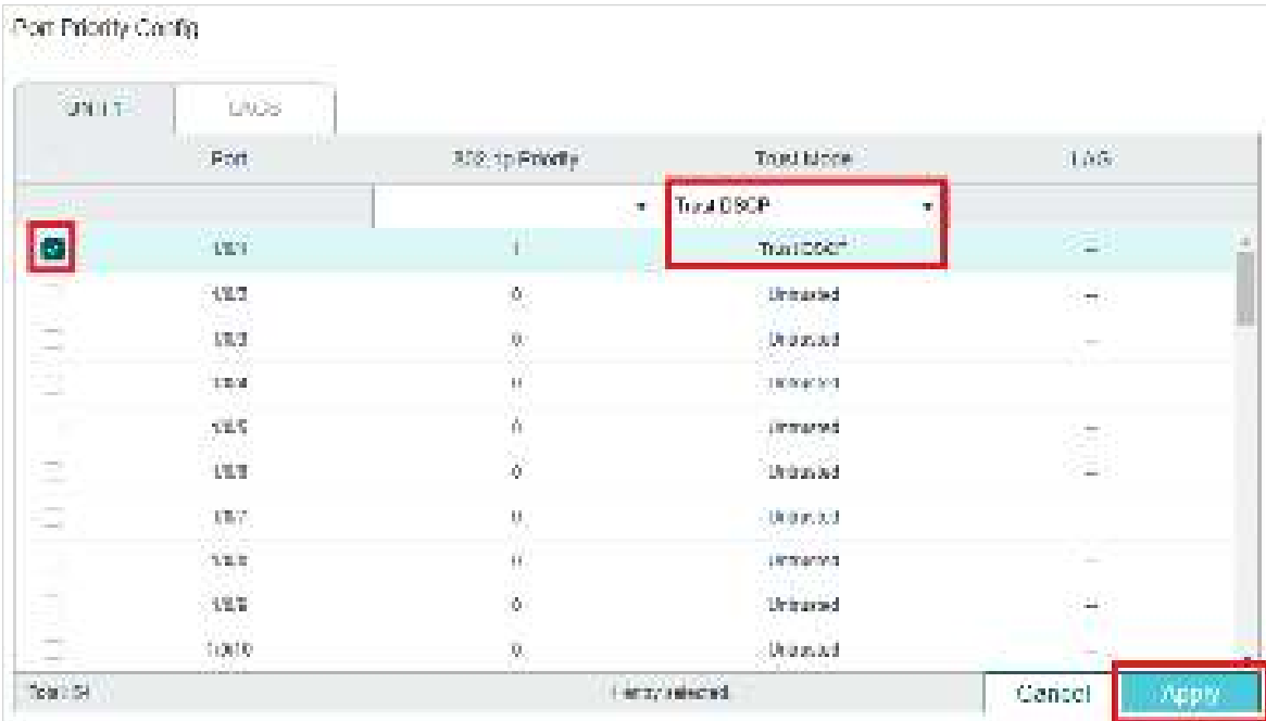
Figure 6-14 Configuring Port Priority
