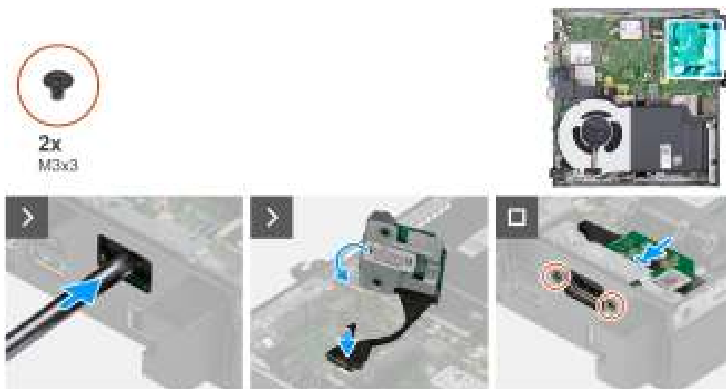
Figure 36. Installing optional I/O module (HDMI, DP, or PS2)
