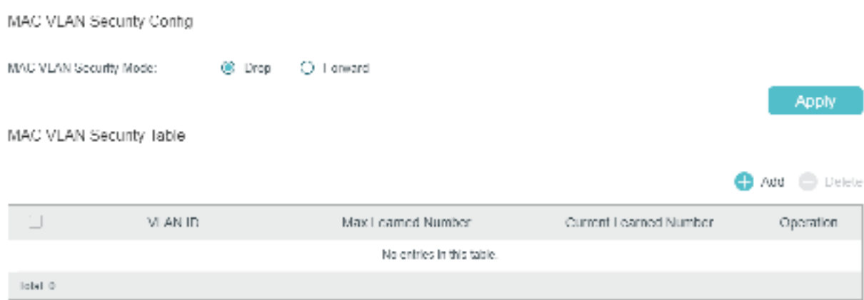
Figure 3-2 Configuring the MAC VLAN Security Mode
