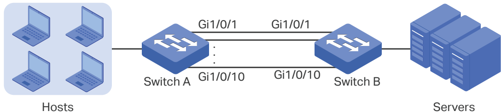
Figure 3-1 Network Topology
