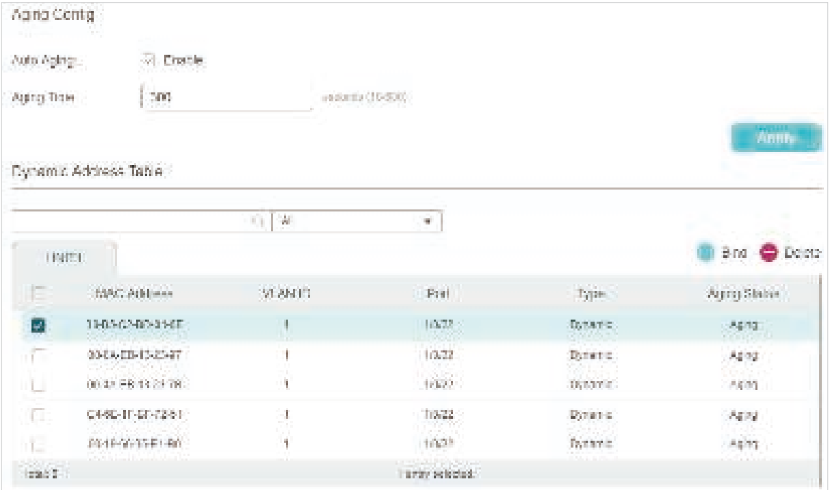
Figure 2-2 Binding Dynamic MAC Address Entries
