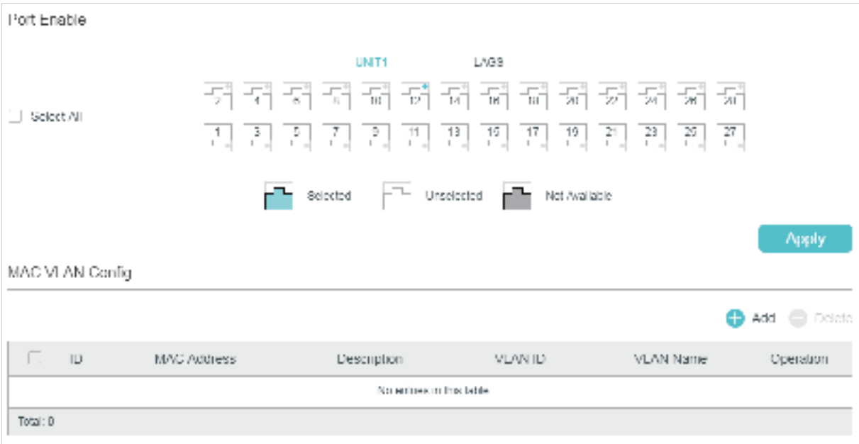
Figure 2-2 Enabling MAC VLAN for the Port
