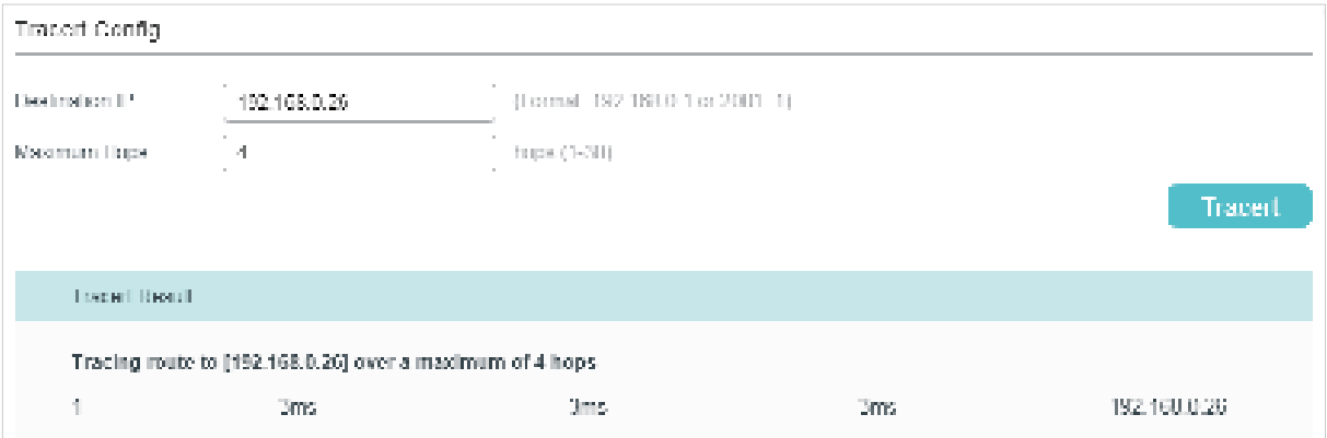
Figure 2-1 Troubleshooting with Tracert Testing
