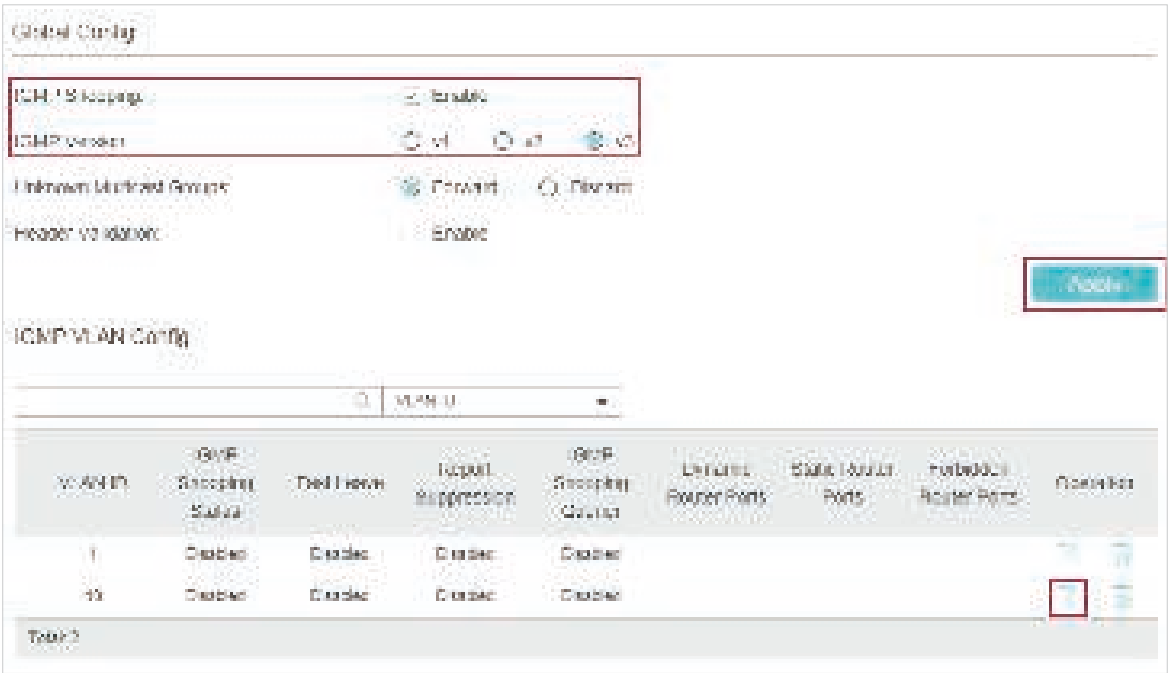
Figure 7-19 Enable IGMP Snooping Globally
