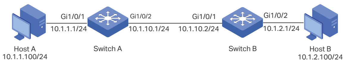
Figure 5-1 Network Topology
