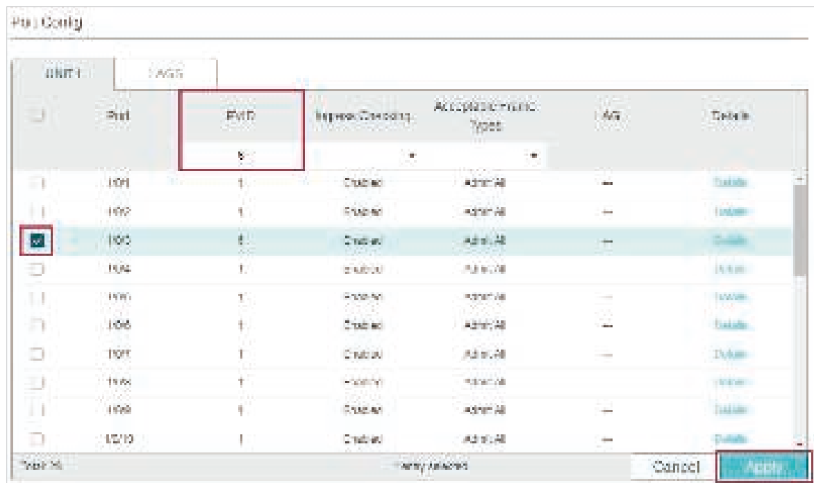
Figure 3-5 Specifying the PVID
