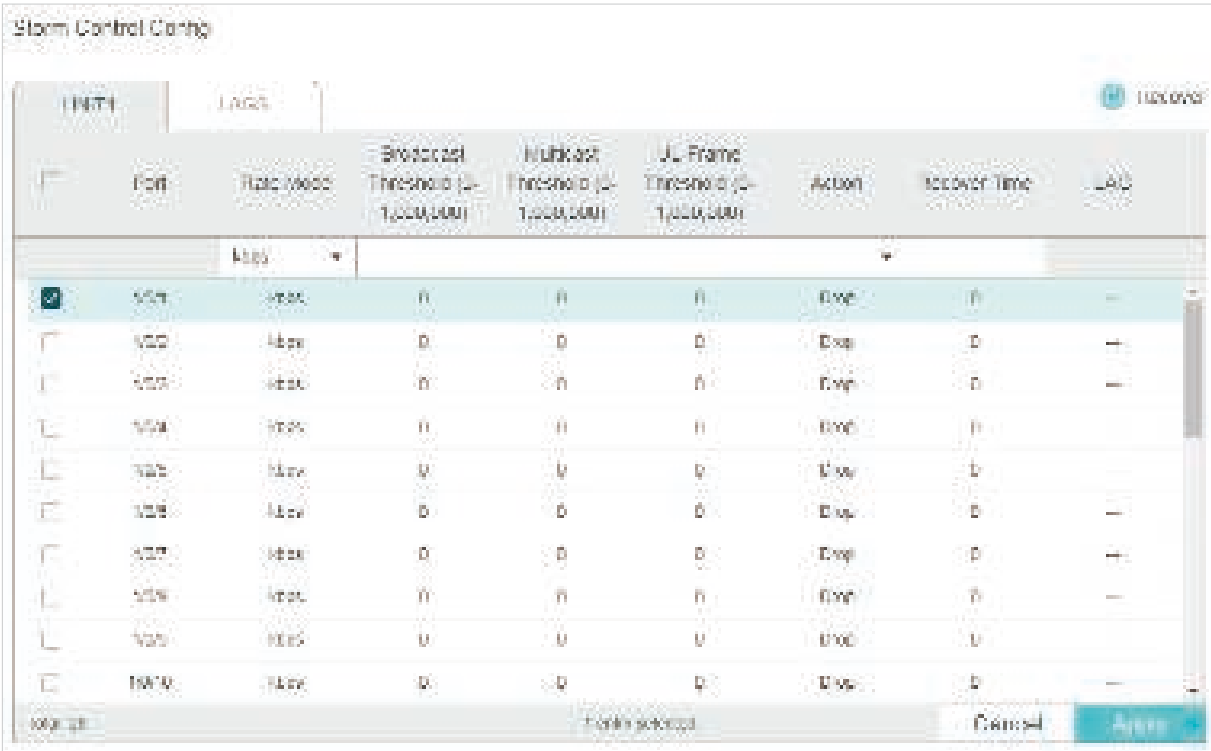
Figure 3-2 Configuring Storm Control
