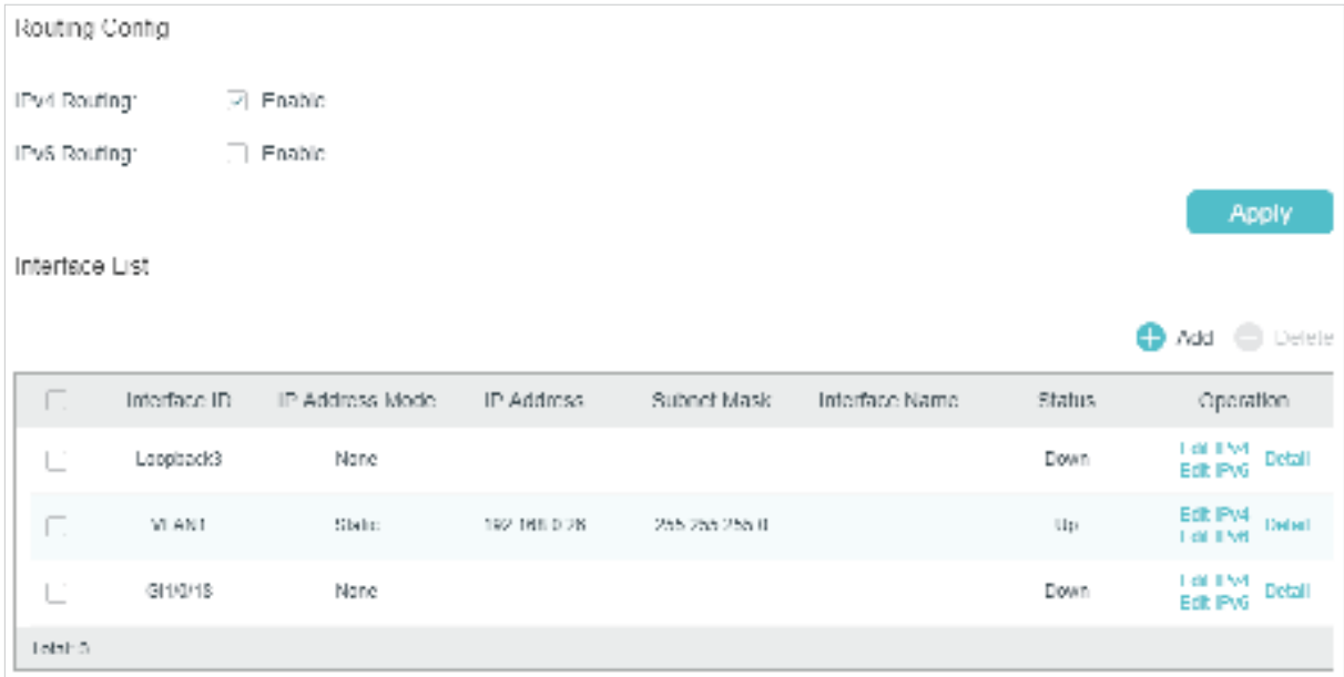
Figure 2-1 Creating an Layer 3 Interface
