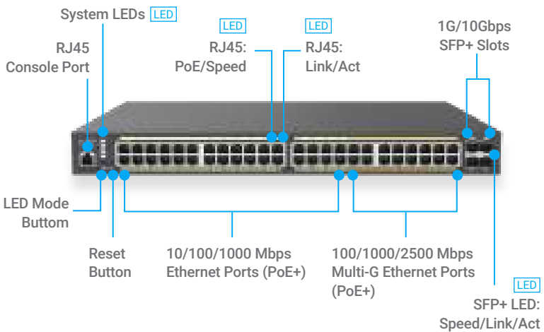
CloudSwitch MGPlus 48 Full PoE (ECS2552FP)
