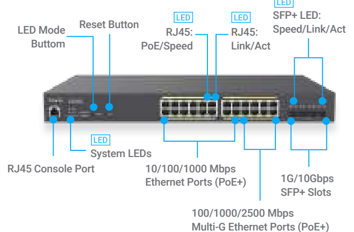
CloudSwitch MGPlus 24 Full PoE (ECS2528FP)
