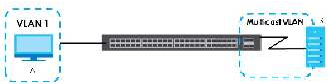
Figure 145 MVR Multicast Television Example
