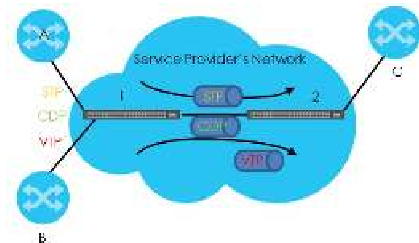
Figure 189 Layer 2 Protocol Tunneling Network Scenario
