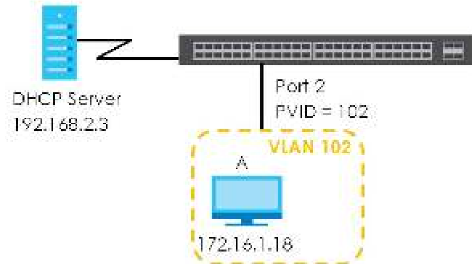
Figure 45 Tutorial: DHCP Relay Scenario
