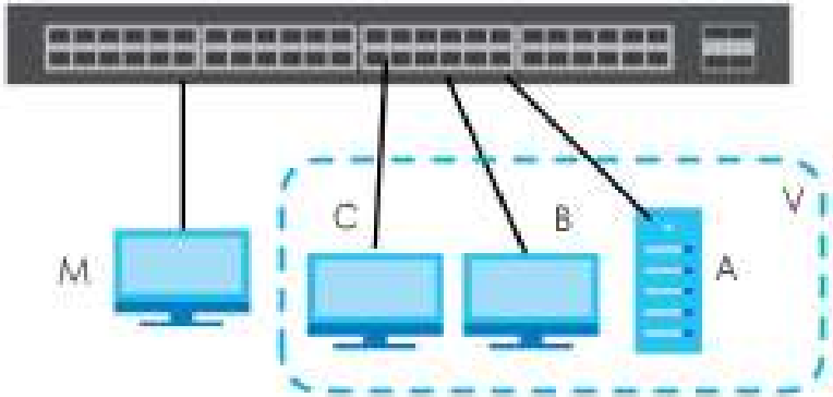
Figure 38 Tutorial: DHCP Snooping Tutorial Overview
