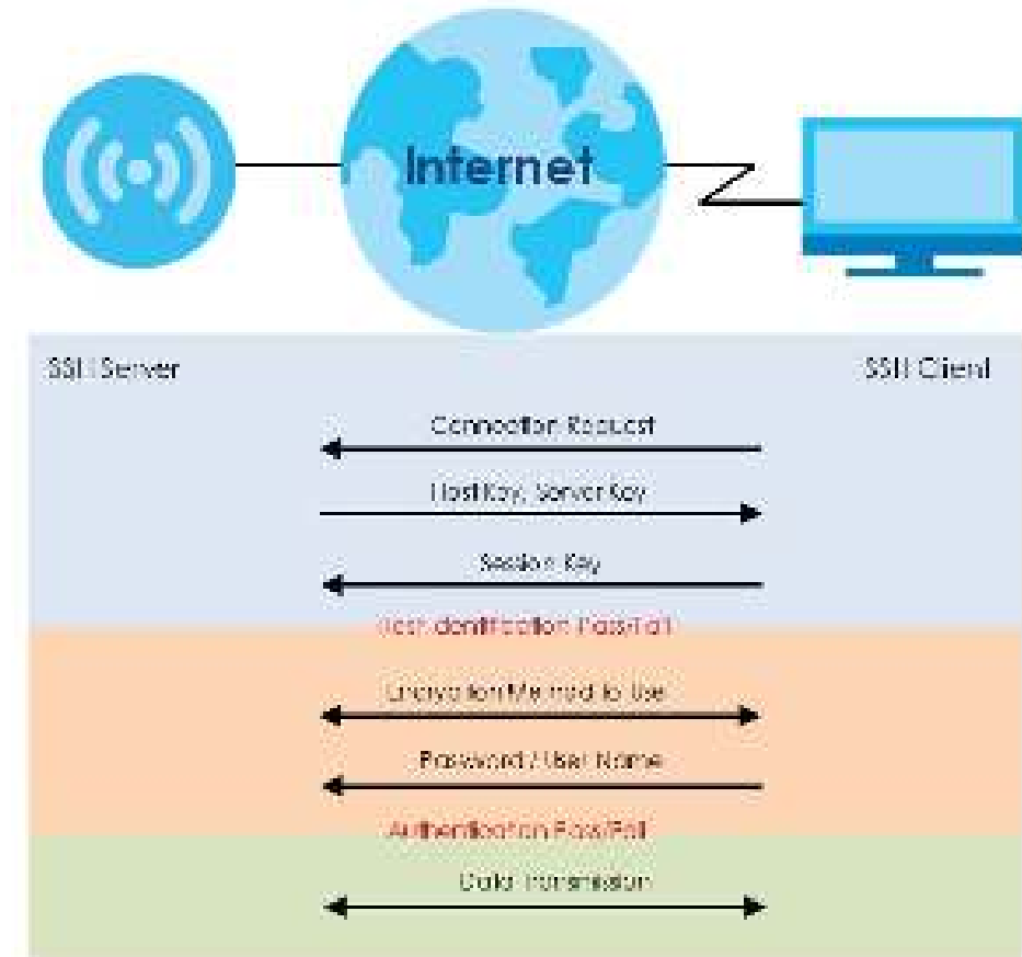
Figure 123 How SSH v1 Works Example
