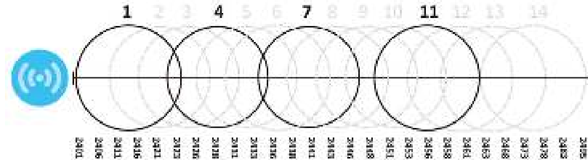
Figure 77 An Example Four-Channel Deployment
