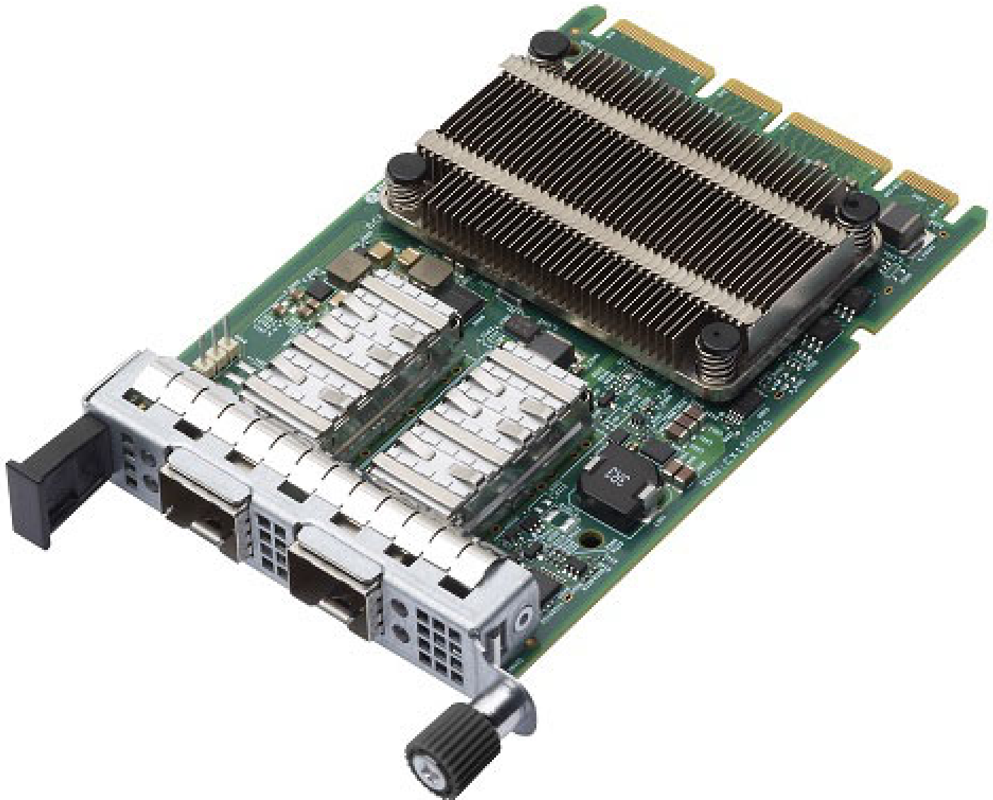
Figure 1: BCM957414N4140C OCP 3.0 SFF Network Adapter
