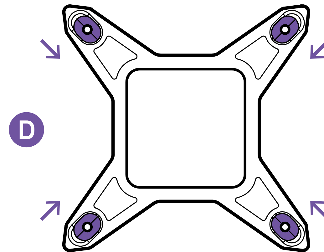
SOCKET 1200/115X
