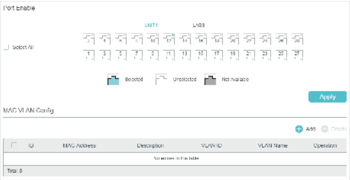
Figure 2-2 Enabling MAC VLAN for the Port
