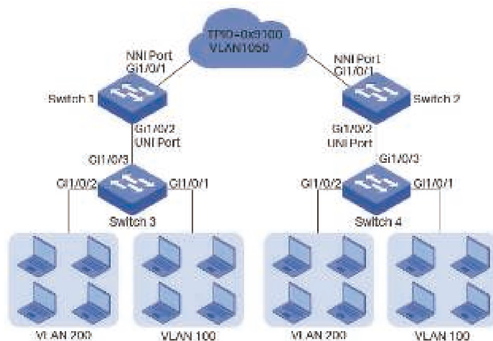
Figure 4-1 Network Topology
