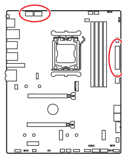
CPU_PWR1~2
