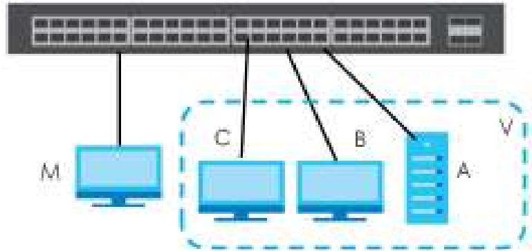
Figure 53 Tutorial: DHCP Snooping Tutorial Overview
