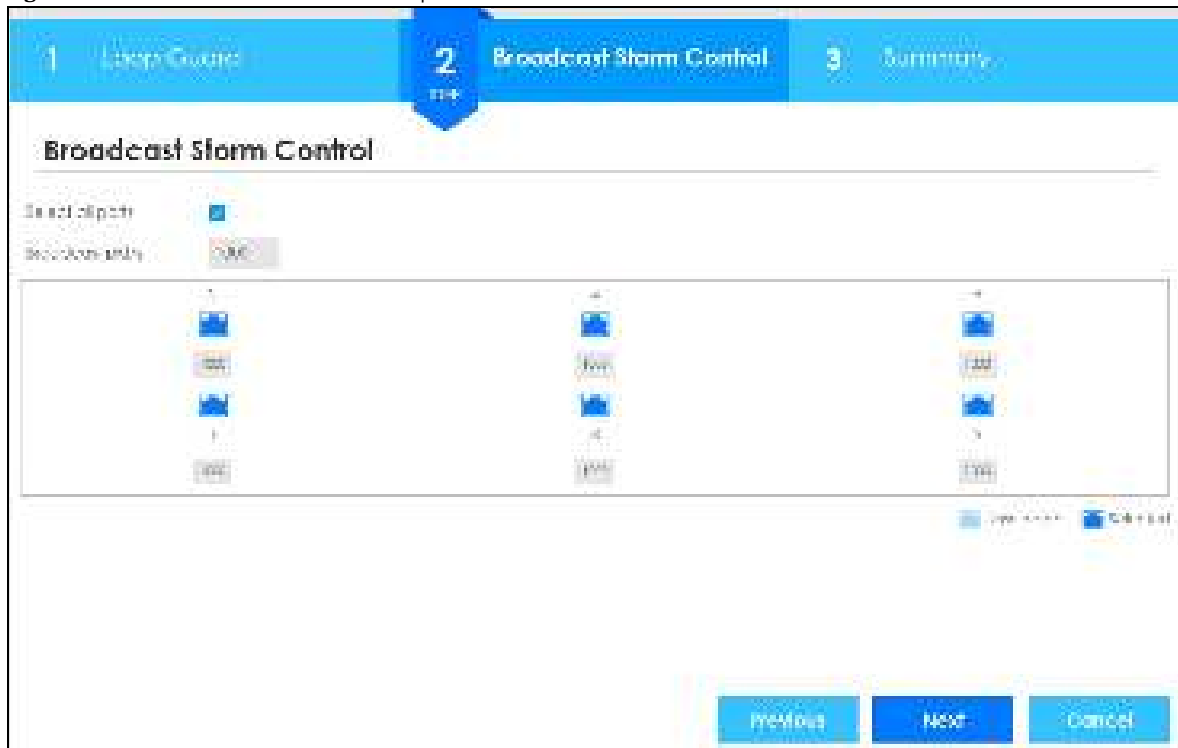
Figure 43 Wizard > Protection > Step 2 Broadcast Storm Control
