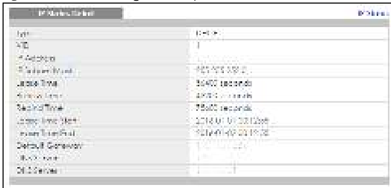
Figure 73 Basic Setting > IP Setup > IP Status Details: DHCP
